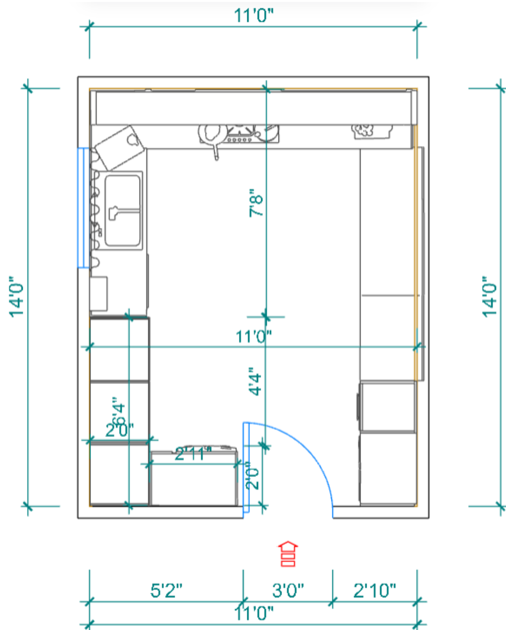
Furniture Size(2/5"=1'-0")
