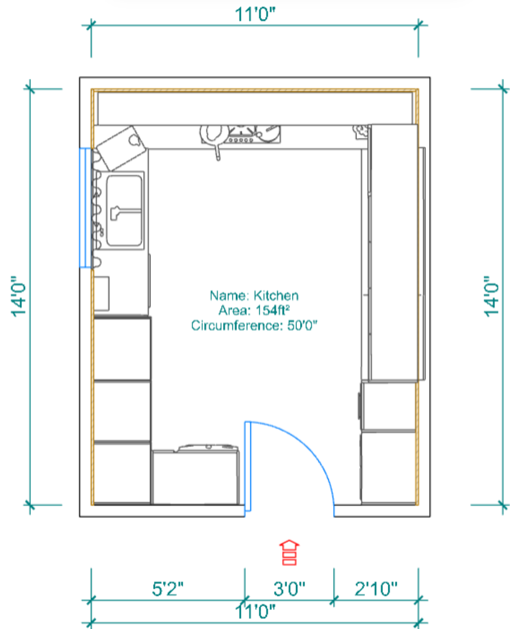
Furniture Plan( 1/3''=1'-0'' )
